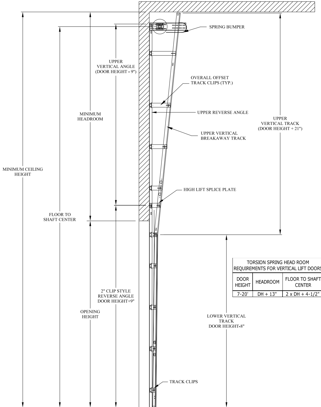
STANDARD VERTICAL LIFT ANGLE MOUNT TRACK SET DETAIL
