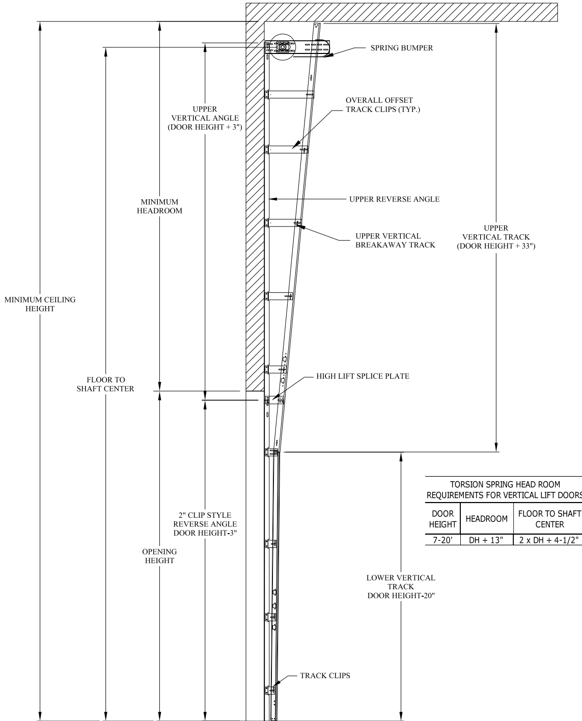
BREAKAWAY VERTICAL LIFT ANGLE MOUNT TRACK SET DETAIL
